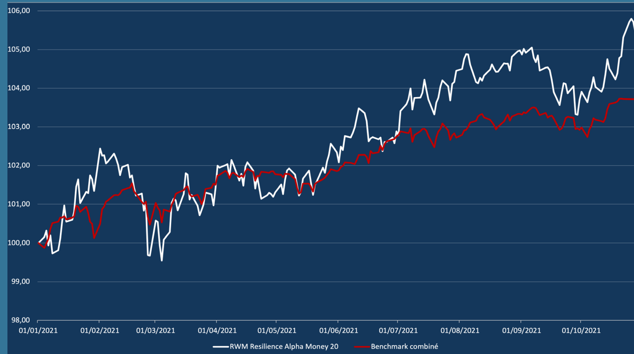
RWM Resilience Alpha Money 20 vs Benchmark combiné*
